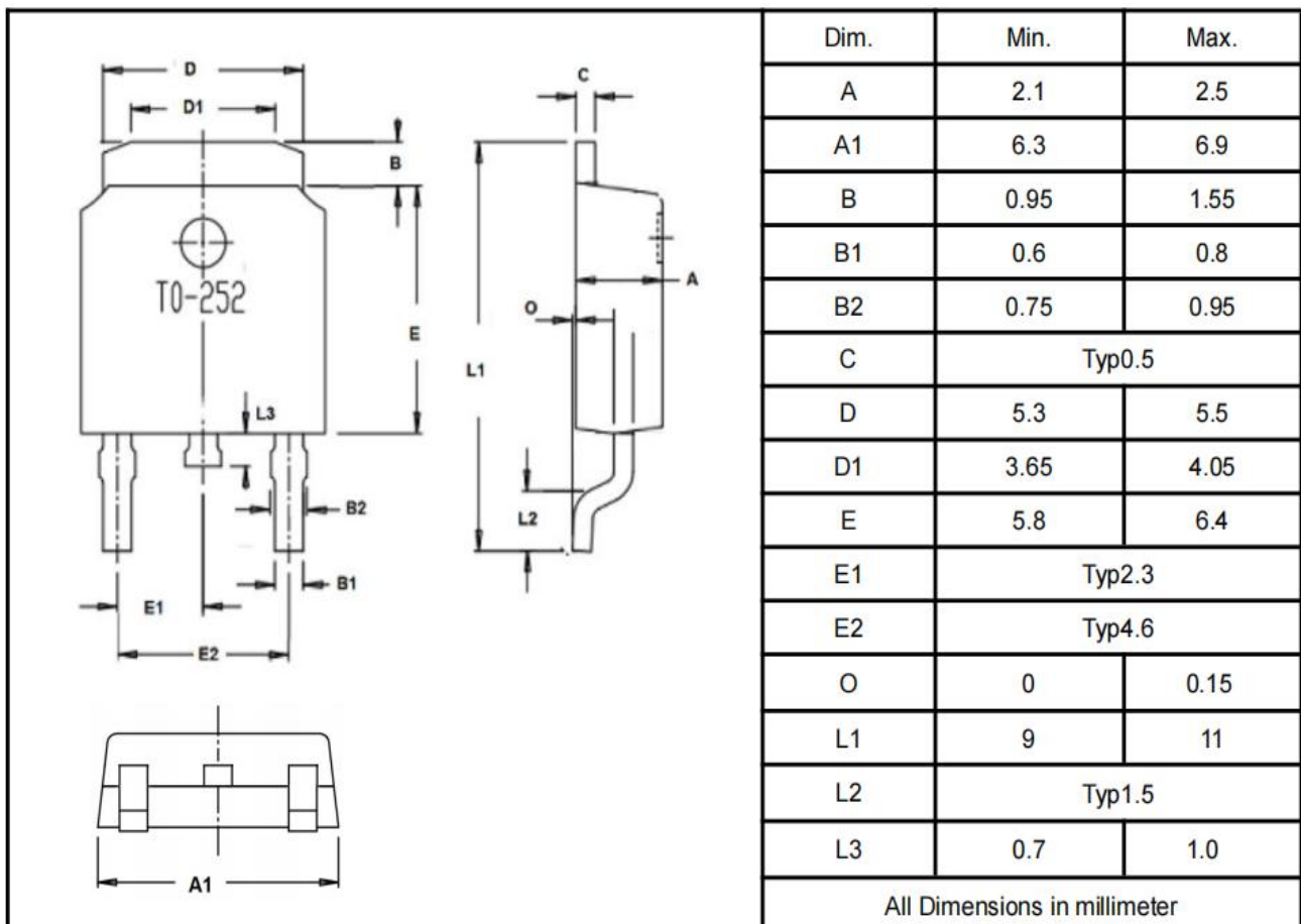
TO-252
